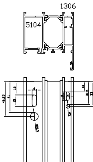
CERCO BALCONERA
