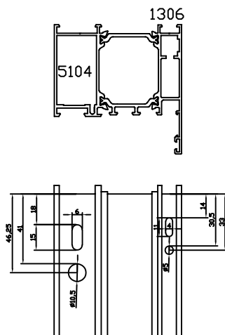
CERCO BALCONERA
