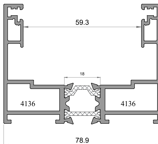
18192M Cerco Perimetral Monocarril Ibiza
