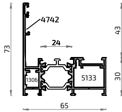
16779L Cerro 30 mm ALG 65 HS
