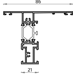
18898L Esquinero Regulable Macho 65 mm
