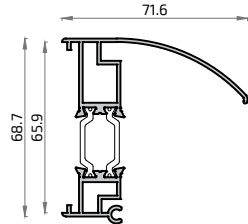
18898L Esquinero Regulable Macho 65 mm
