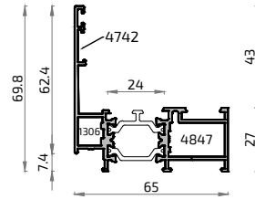
16764L NO STOCK Cerro 27 mm ALG 65 HS
