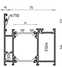
16300H Cerro ALG 75
