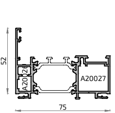
18973H NO STOCK Cerro Garganta ALG 75
