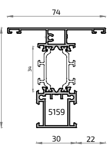
16308H NO STOCK Pilastra Reforzada ALG 75
