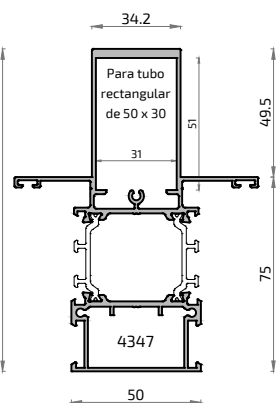
16308H NO STOCK Pilastra Reforzada ALG 75
