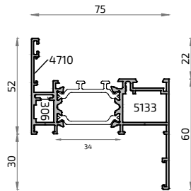
17435H NO STOCK Cerro Ventana C/Solape 30 mm ALG 75
