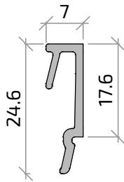
21248 Junquillo 7 x 17.5 mm
