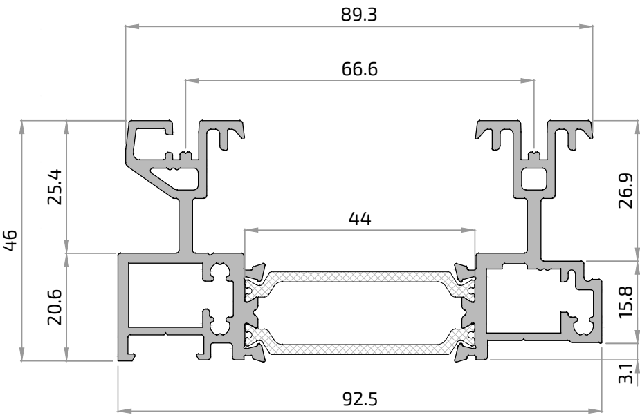
21676P Cerco Base multicarril Matra NG*
