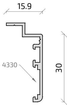
8832 Solapa Inf. Monoblock 30 mm
