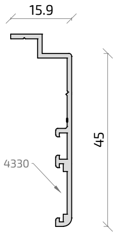
8630 Solapa Inf. Monoblock 45 mm
