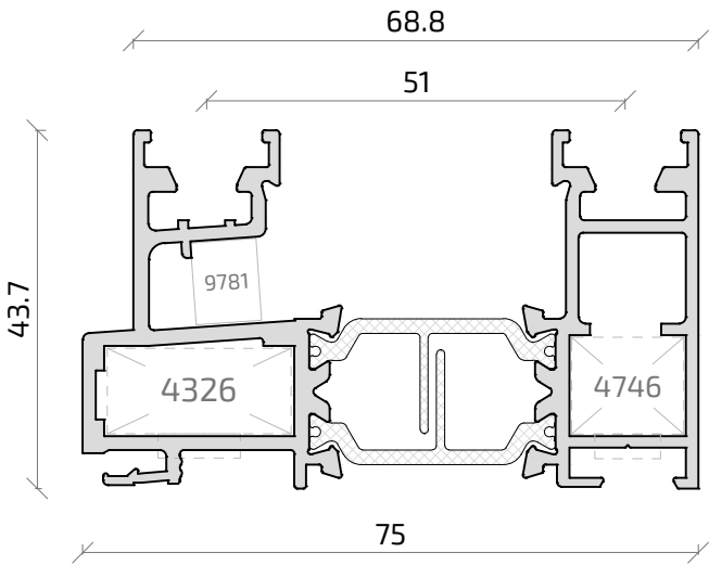
18143L NO STOCK Cerco 2C Alg Slide 75 clip+grapa
