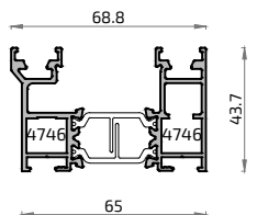
18131L Cercos 75 grapa+grapa
