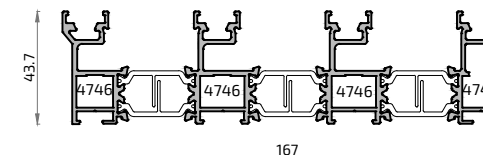
20655L NO STOCK Cercos 5 carriles grapa+grapa
