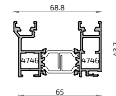
18147L Cercos 75 grapa+clip
