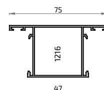
119 2552 Pilastra 47 mm S-100
