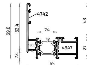
16764L NO STOCK Cercos 27 mm ALG 65 HS
