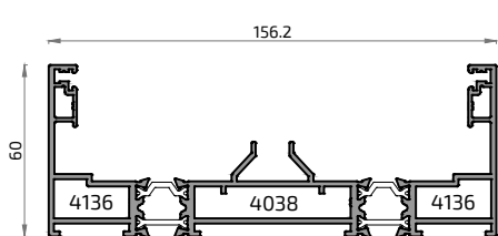
20601M Cercos Desmontable 2 Carriles Ibiza
