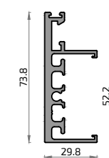
10964 Hoja Central Ibiza
