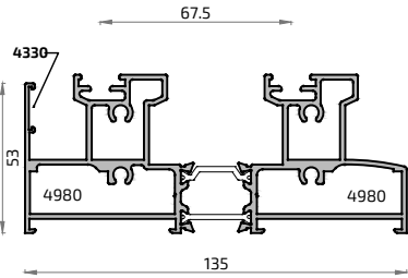
8670M 1160M Cercos 2 Carriles Matra 135 RPT
