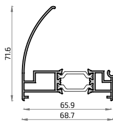
18898L Esquinero regulable macho 65
