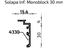
775 3596 Solapa Inf. Monoblock 30 mm
