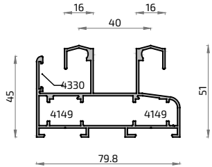
8597 Cercos Perimetral 80 mm Silver 76
