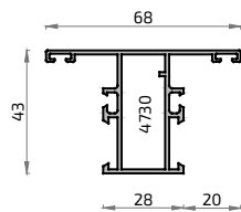
8860 Pilastra Cercos 28 mm Silver 76
