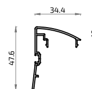
8596 Acople Central Curvo Silver 76
