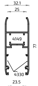
8586 Hoja Perimetral 77 mm Silver 76
