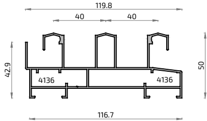
8578 Cercos 3 Carriles Silver 76
