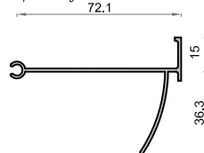
610 6115 Esquinero Regulable Macho
