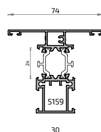
16339L Pilastra 30 mm ALG 65
