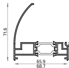
18898L Esquinero Regulable Macho ALG 65
