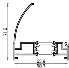
18898L Esquinero Regulable Macho ALG 65
