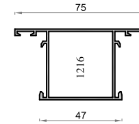
119 2552 Pilastra 47 mm S-100
