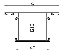
119 2552 Pilastra 47 mm S-100
