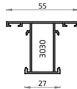
113 2546 Pilastra Lisa 27 mm S-100
