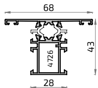
8865M Pilastra 28 mm Silver 65RPT
