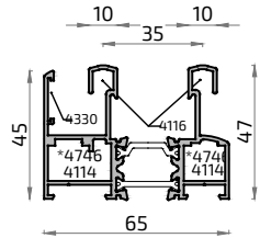
10000M Cercos Perimetral 65 mm Silver 65RPT
