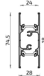
10005M Partelunas Silver 65RPT
