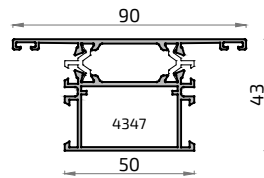
8810M Pilastra 50 mm Silver 65RPT
