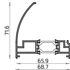
18898L Esquinero regulable macho 65
